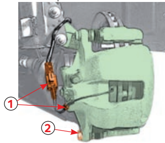
Brake caliper lower retainer removal
