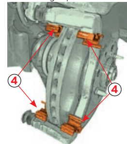
Sliding clip removal
