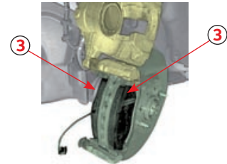
Brake shoe removal
